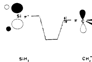
Figure 2. Orbital interaction between CH_2^- and the \alpha -silyl fragment.
